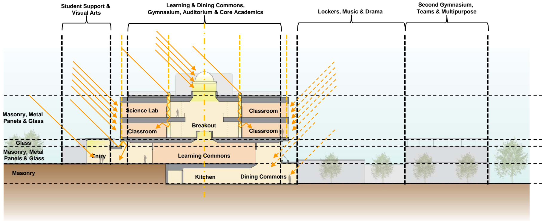
Section through Learning Commons
