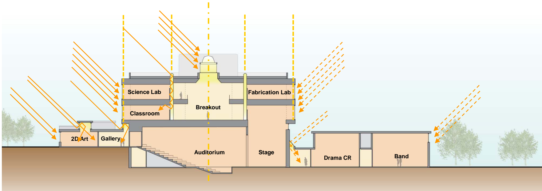
Section through Auditorium
